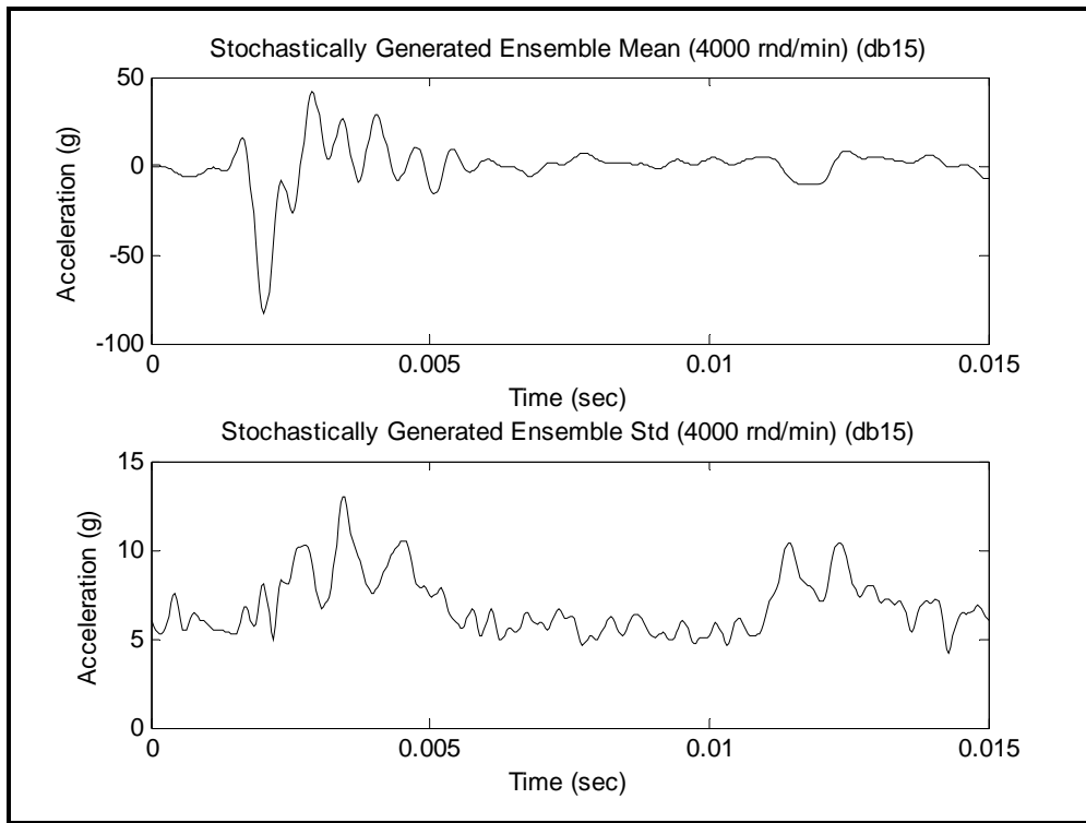
Figure 519.6B-8d. Ensemble and stochastically generated pulse ensemble random component standard deviation (4000 r/min)
