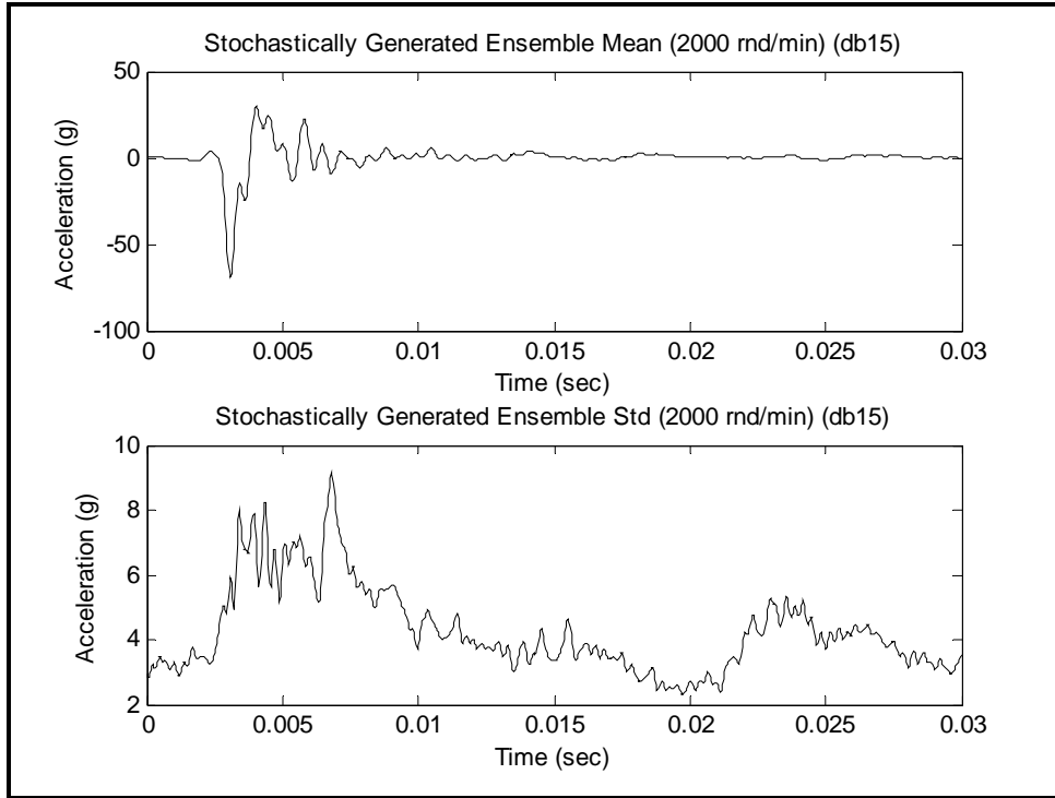
Figure 519.6B-8c. Ensemble and stochastically generated pulse ensemble random component standard deviation (2000 r/min).
