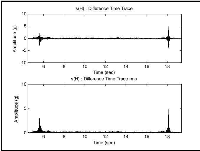
Figure 525A-9a. Difference Exciter (H)
