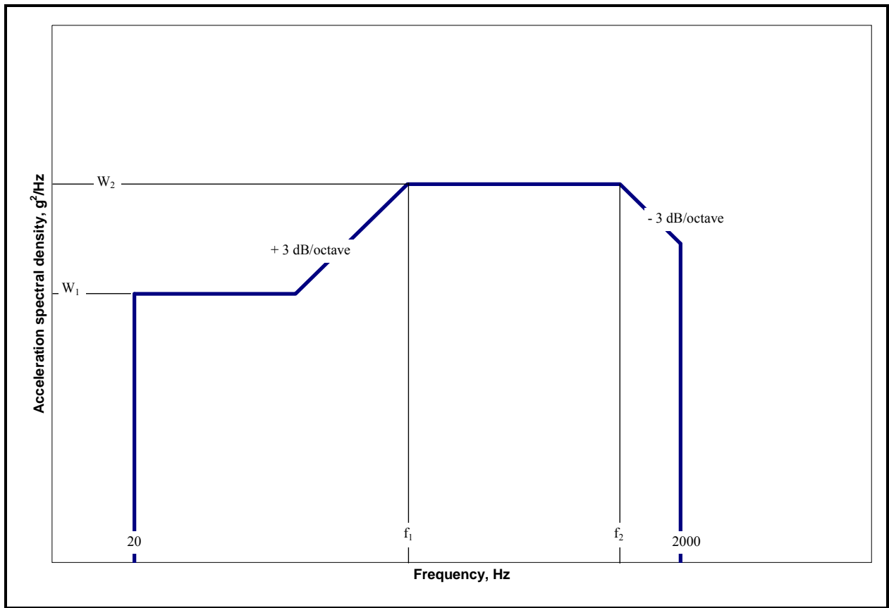
Figure 514.6D-7. Category 16 - Jet aircraft store equipment vibration exposure.
